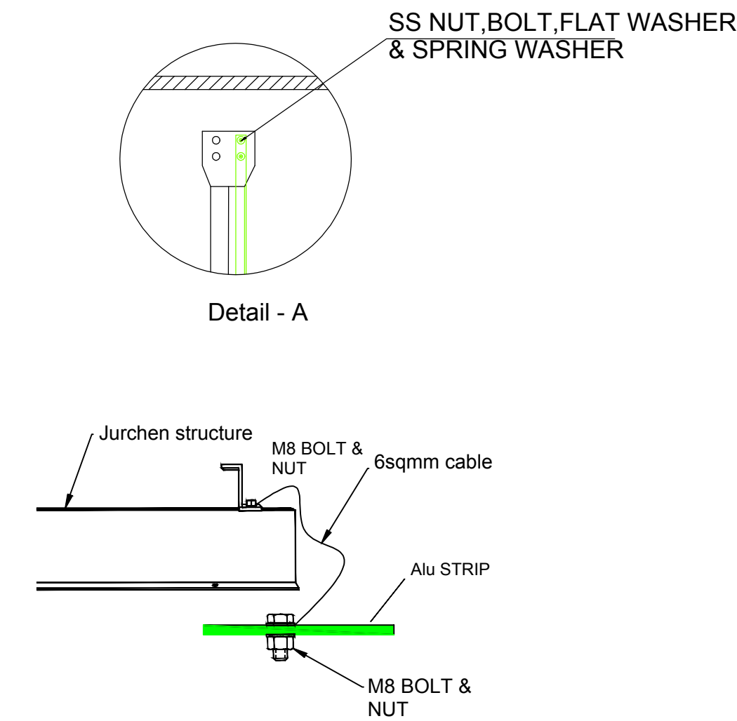
JOINTING DETAIL OF ALU STRIP
